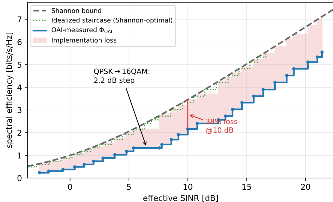
OAI-measured link curve vs. Shannon bound
