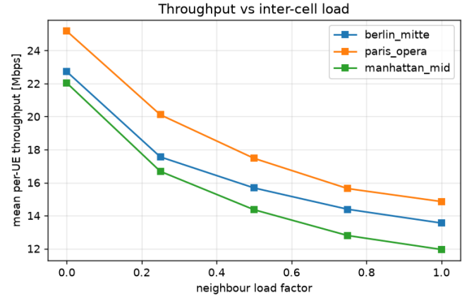
Fig. 6. Mean per-UE throughput vs. inter-cell load factor, per scene. Served users are interference-limited.
