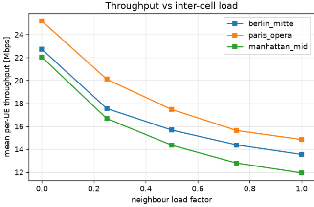
Fig. 7. Mean per-UE throughput vs. inter-cell load factor, per scene. Served users are interference-limited.
