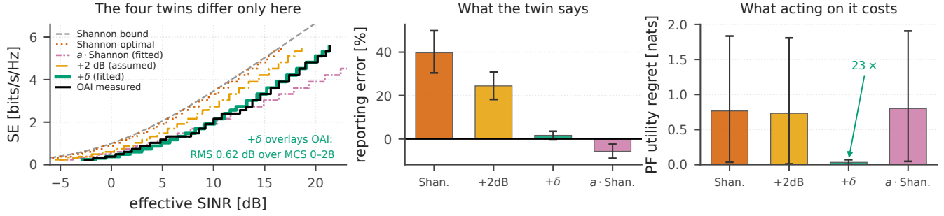
Fig. 2. Left: the four twins share one (MCS, SE) set and differ only in the SINR at which each MCS unlocks; the fitted-offset curve overlays the OAI staircase (0.62 dB RMS), while the fitted attenuation tracks it on average and diverges at both ends. Centre, right: reporting error and regret, means with seeded bootstrap 95% CIs over 24 runs. The two are close to independent—the attenuation model reports best of the three surrogates and acts worst.
