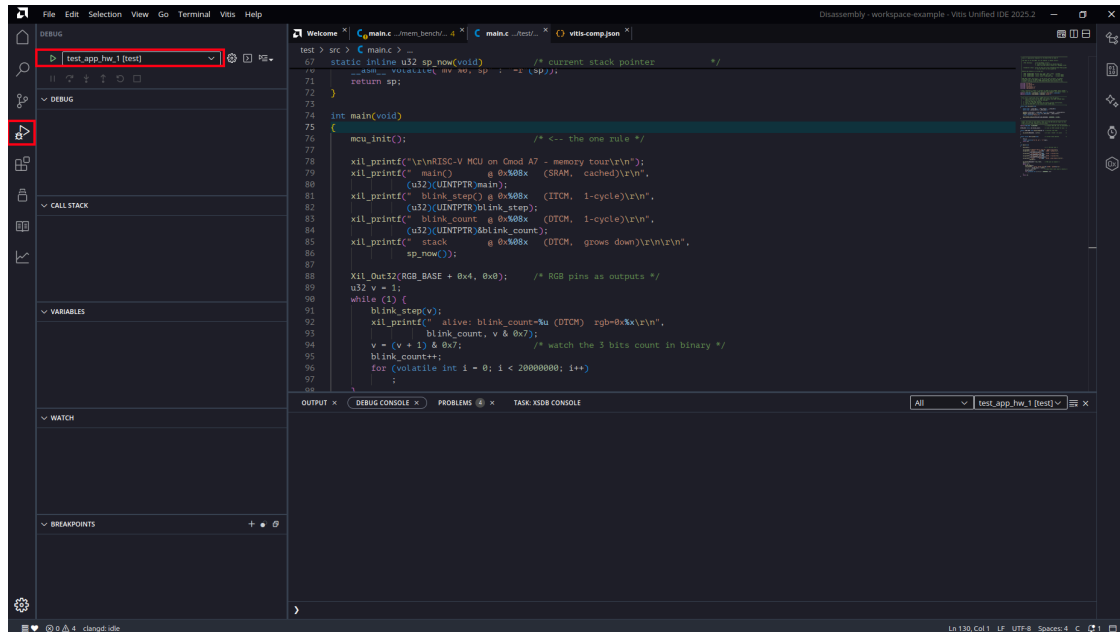
Figure 33: Debug Launched
