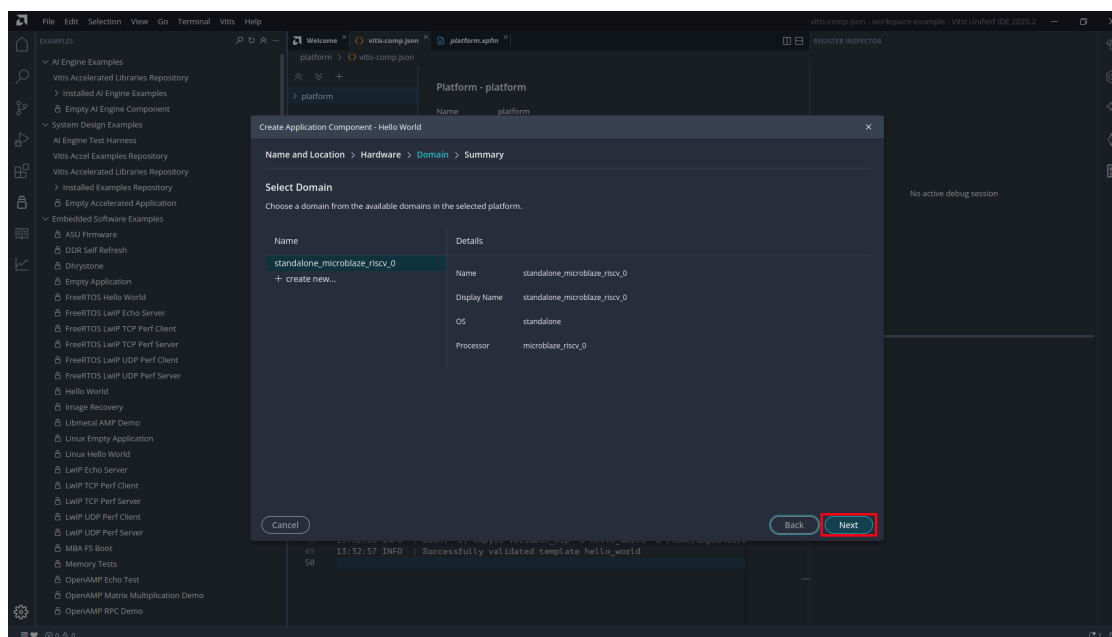
Figure 22: Select Domain
