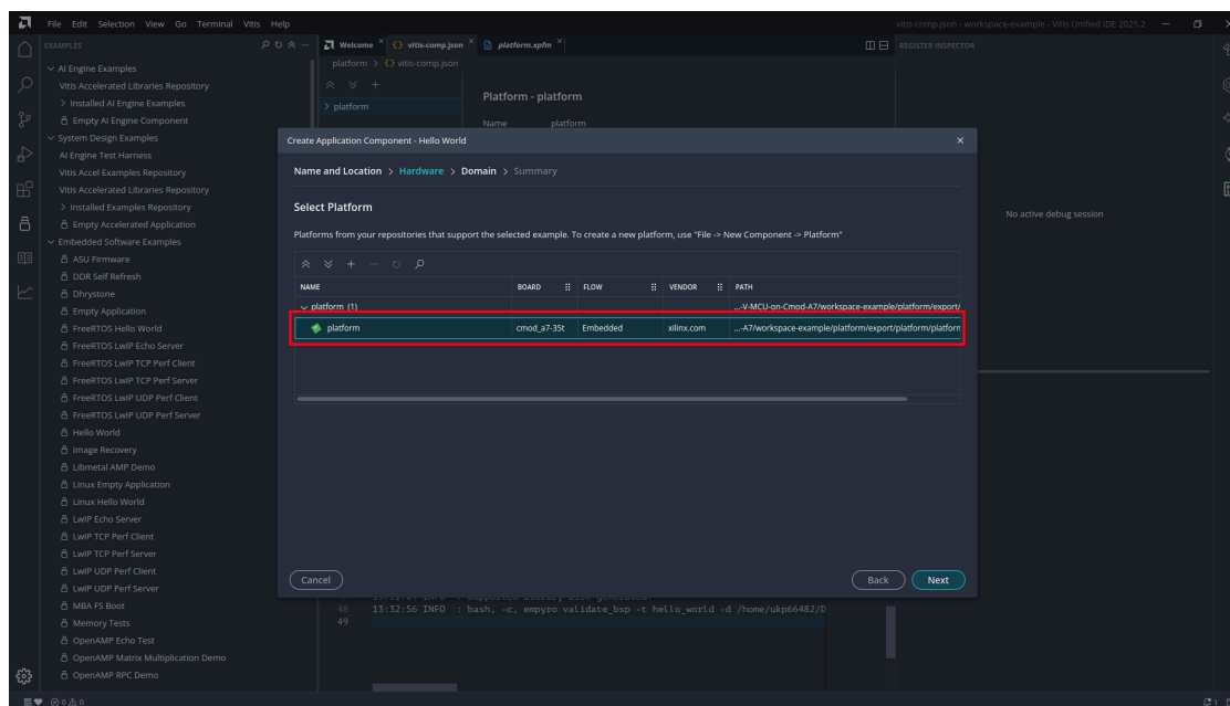
Figure 21: Select Platform
