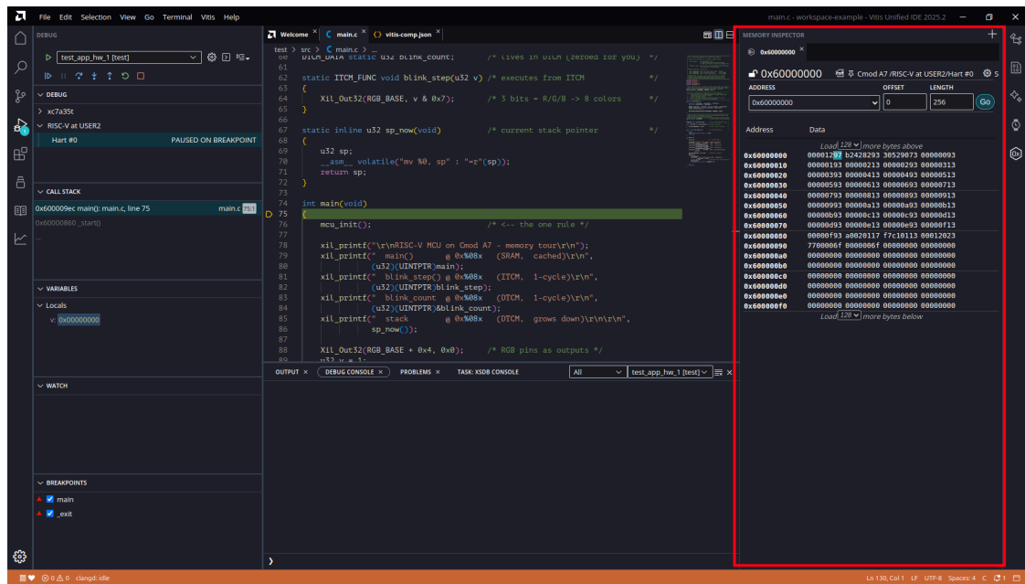
Figure 39: Memory Inspector
