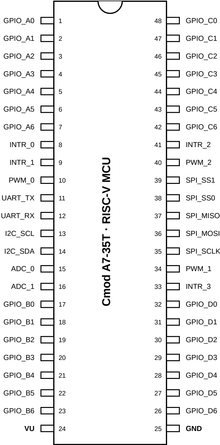
top view · 48-pin DIP · LVC MOS33 (pins 15/16 analog via divider)
