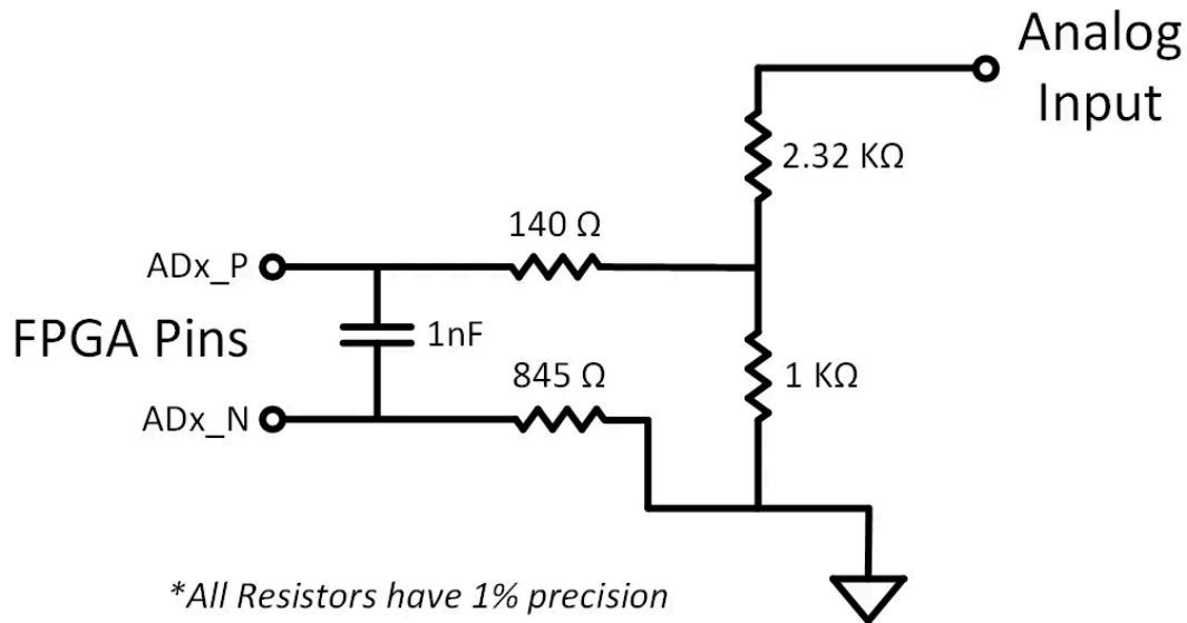
Figure 3: On-board voltage divider circuit for XADC analog inputs (from Diligent Reference Manual)
