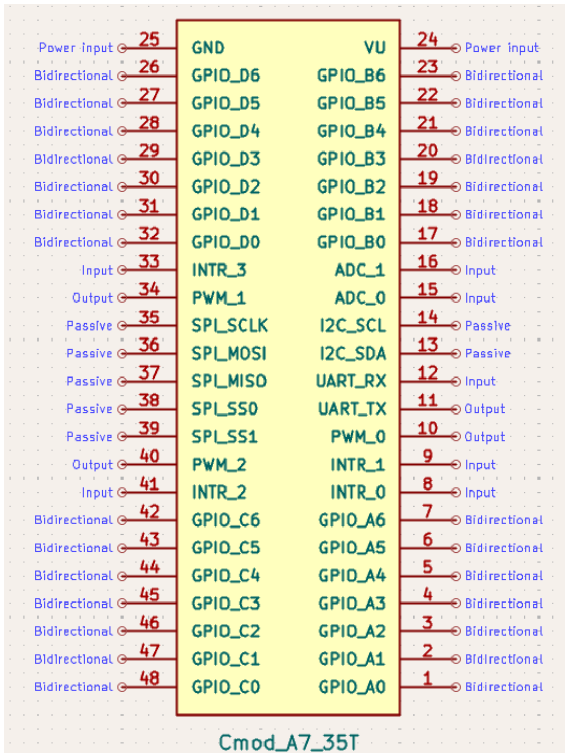
Figure 2: U1 Cmod A7-35T DIP Pinout (custom schematic symbol)
