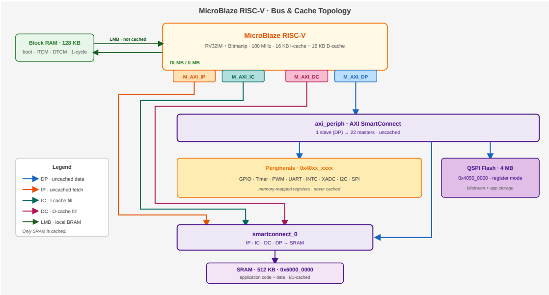
Figure 1: Bus & Cache Topology
