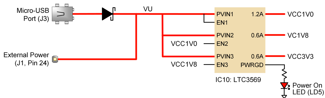
Figure 4: Cmod A7 Power Supply (from Digilent Reference Manual)
