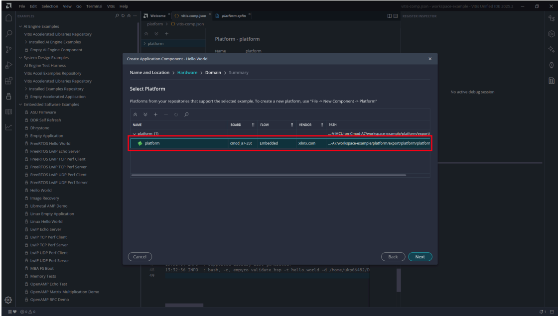
Figure 37: Select Platform
