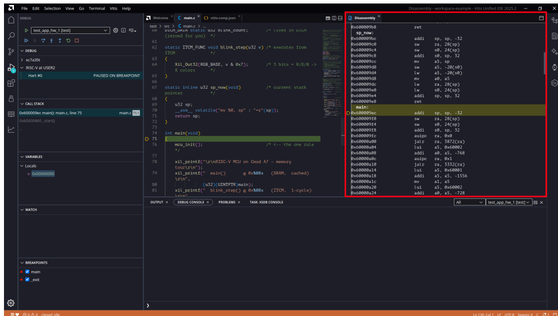
Figure 56: Disassembly
