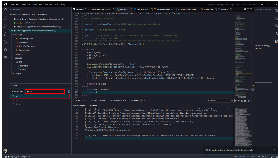
Figure 47: Build Application
