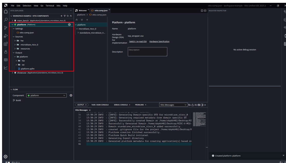
Figure 34: Platform Created
