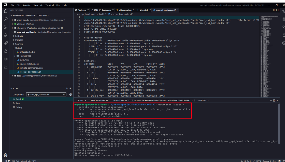
Figure 70: updatemem in the Integrated Terminal
