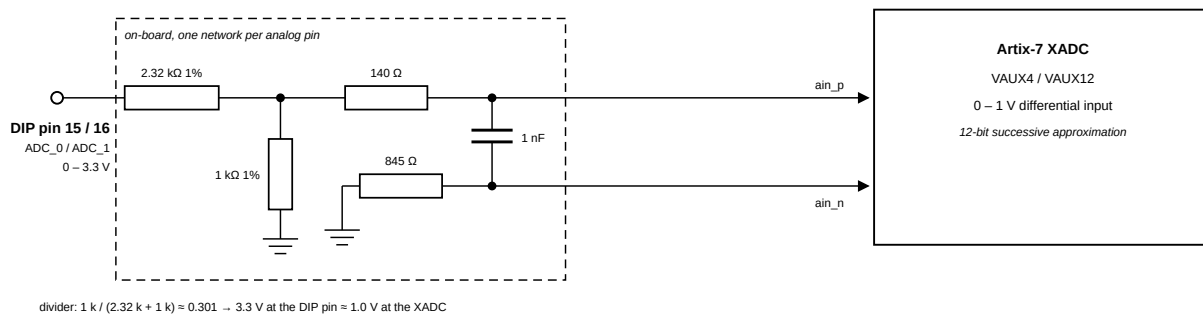
Figure 22: On-board voltage divider circuit for XADC analog inputs
