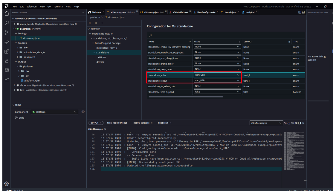
Figure 45: stdin/stdout Set to uart_USB
