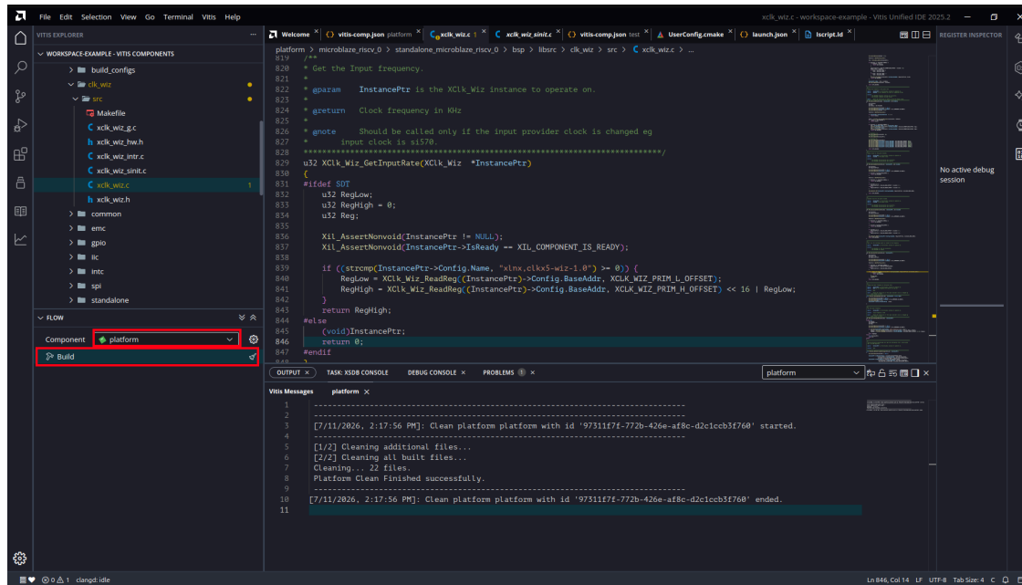
Figure 46: Build Platform
