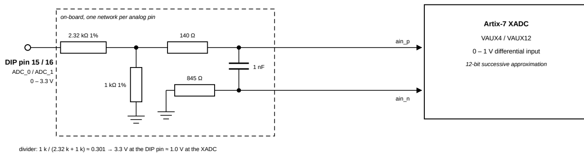
Figure 31: On-board voltage divider circuit for XADC analog inputs
