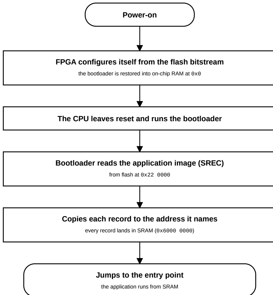
Figure 68: Standalone boot sequence: the FPGA restores the bootloader, which copies the application from flash into SRAM and runs it
