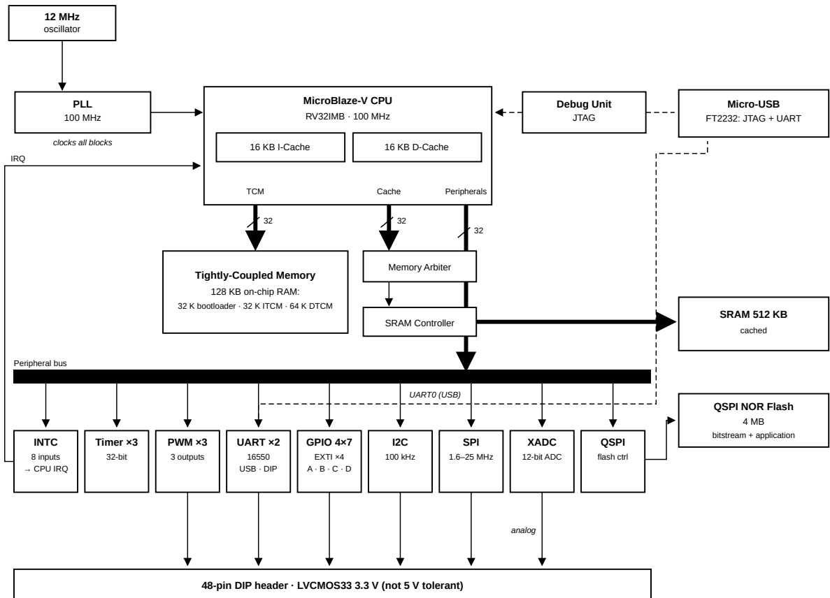
Figure 1: System Architecture
