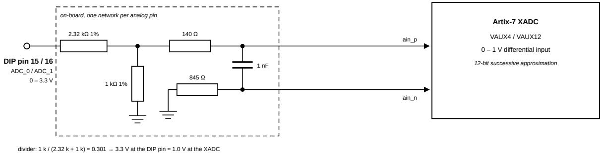
Figure 7: On-board voltage divider circuit for XADC analog inputs
