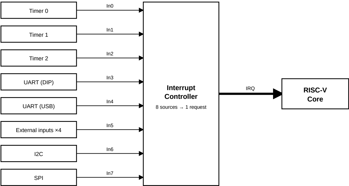
Figure 3: The interrupt controller collects eight sources into one request to the core
