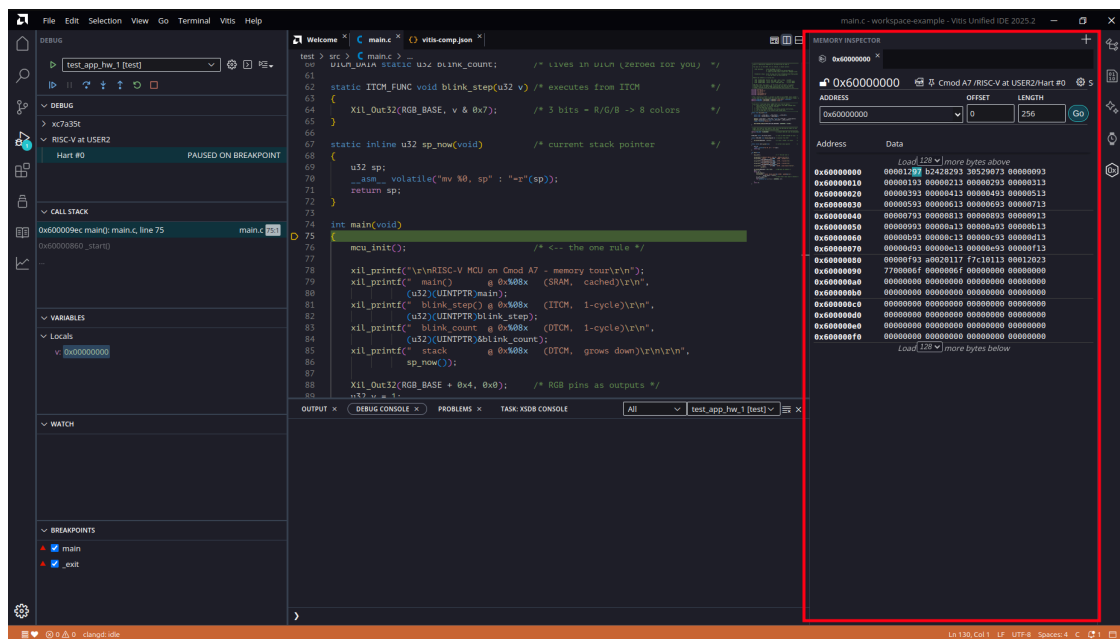
Figure 38: Memory Inspector
