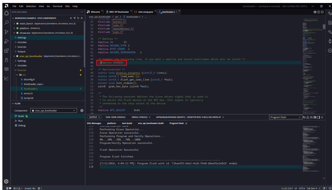
Figure 50: VERBOSE Disabled
