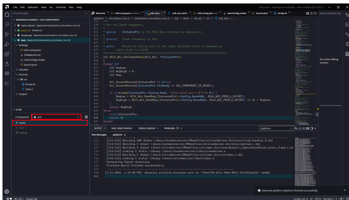
Figure 31: Build Application
