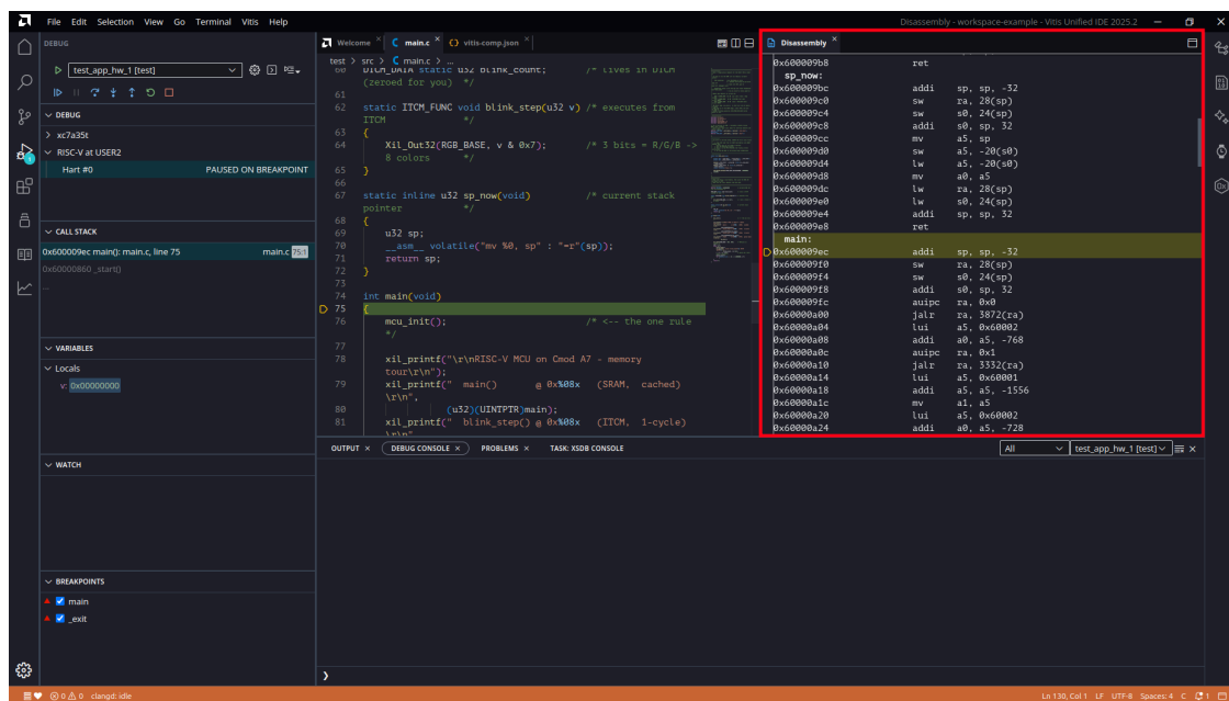
Figure 40: Disassembly
