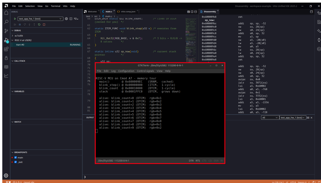
Figure 45: Memory Tour and Status Output
