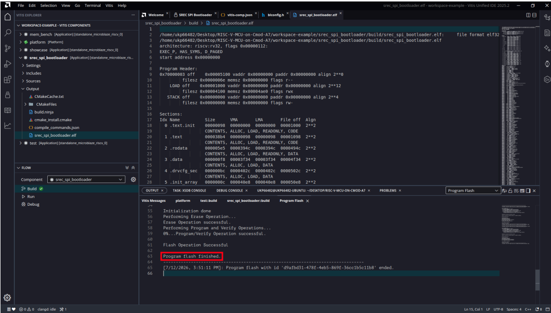
Figure 70: Application Slot Programmed
