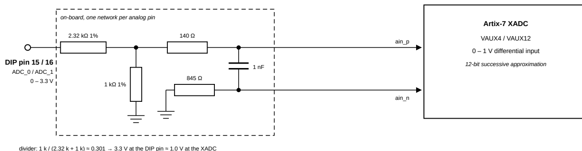
Figure 17: On-board voltage divider circuit for XADC analog inputs
