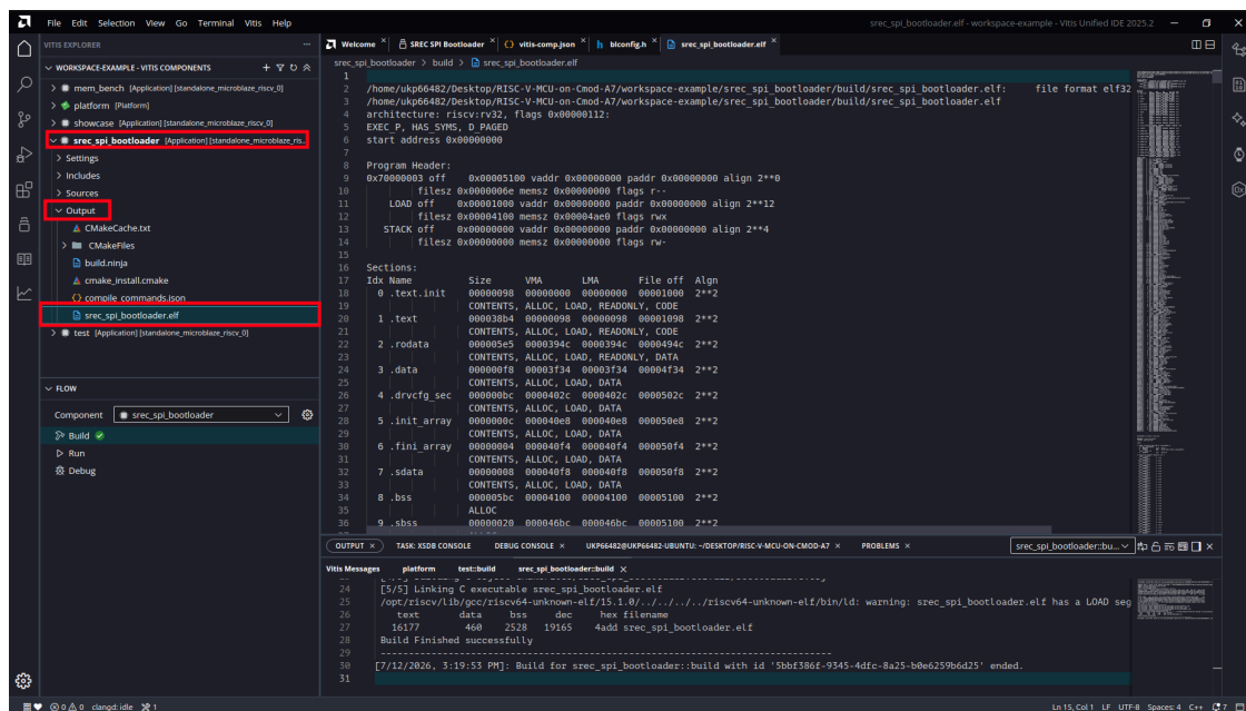
Figure 62: Bootloader ELF Built
