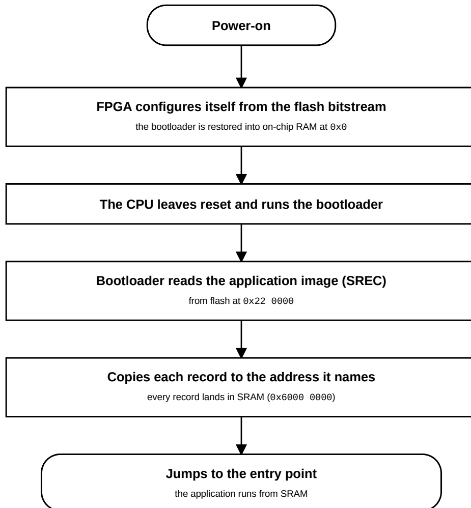
Figure 52: Standalone boot sequence: the FPGA restores the bootloader, which copies the application from flash into SRAM and runs it
