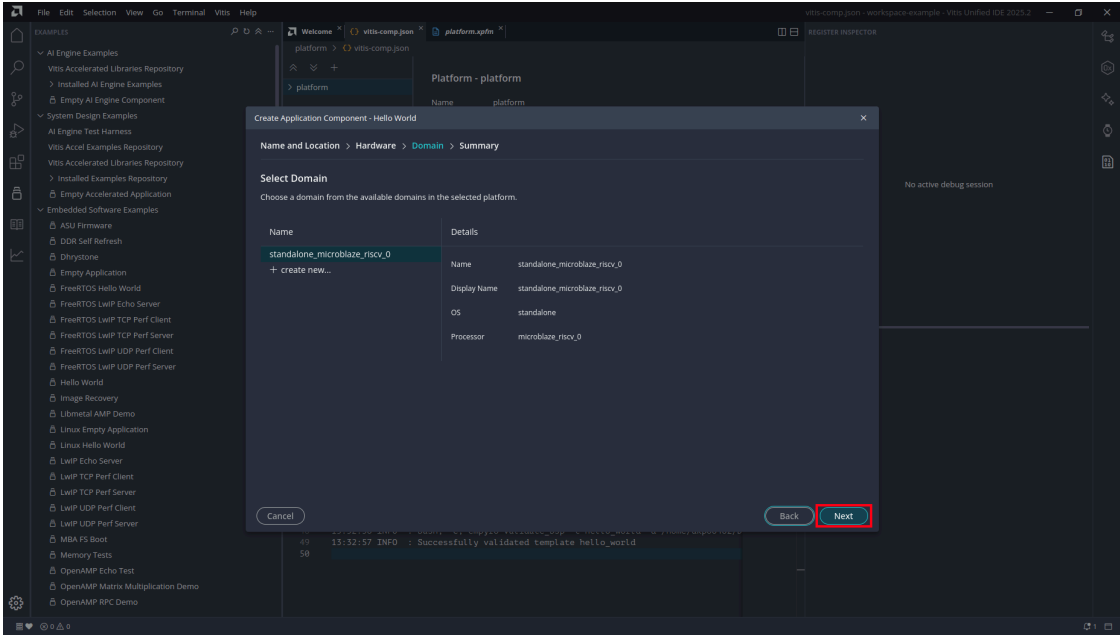
Figure 31: Select Domain
