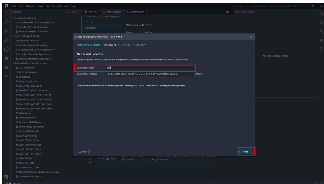
Figure 29: Application Name
