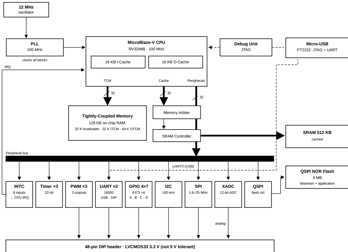
Figure 1: System Architecture
