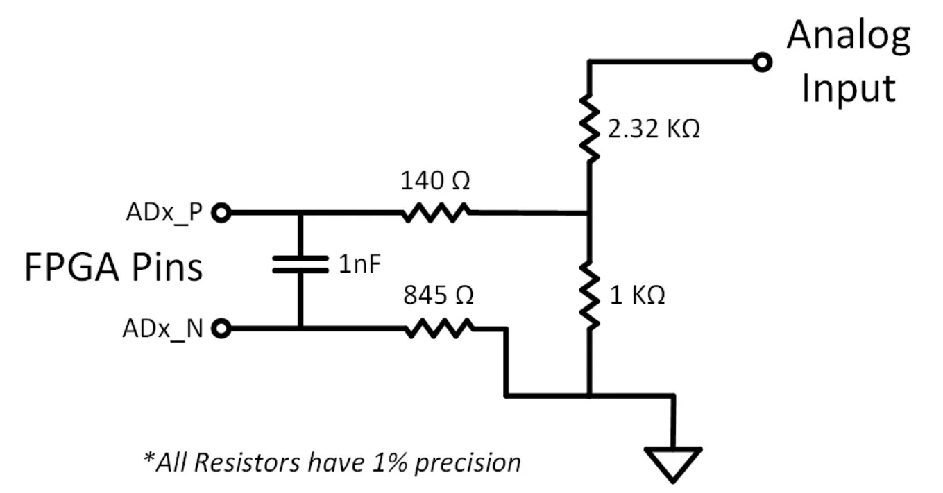
Figure 2. On-board voltage divider circuit for XADC analog inputs (from Digilent Reference Manual)
