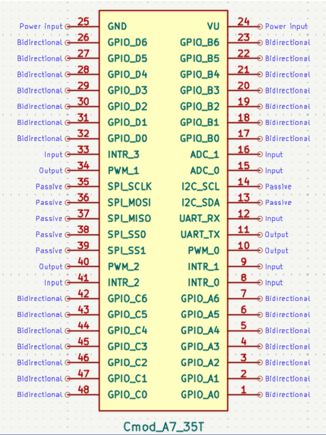
Figure 1. U1 Cmod A7-35T DIP Pinout (custom schematic symbol)
