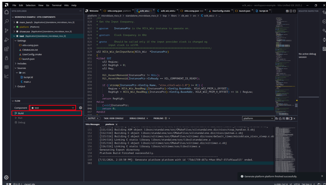
Figure 31: Build Application
