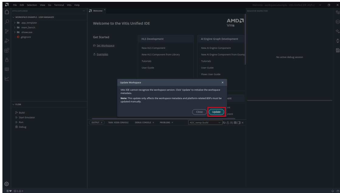
Figure 11: Update Workspace
