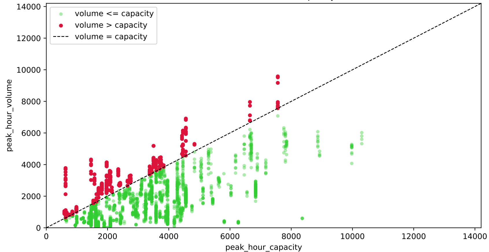
Peak Hour Volume vs. Capacity
