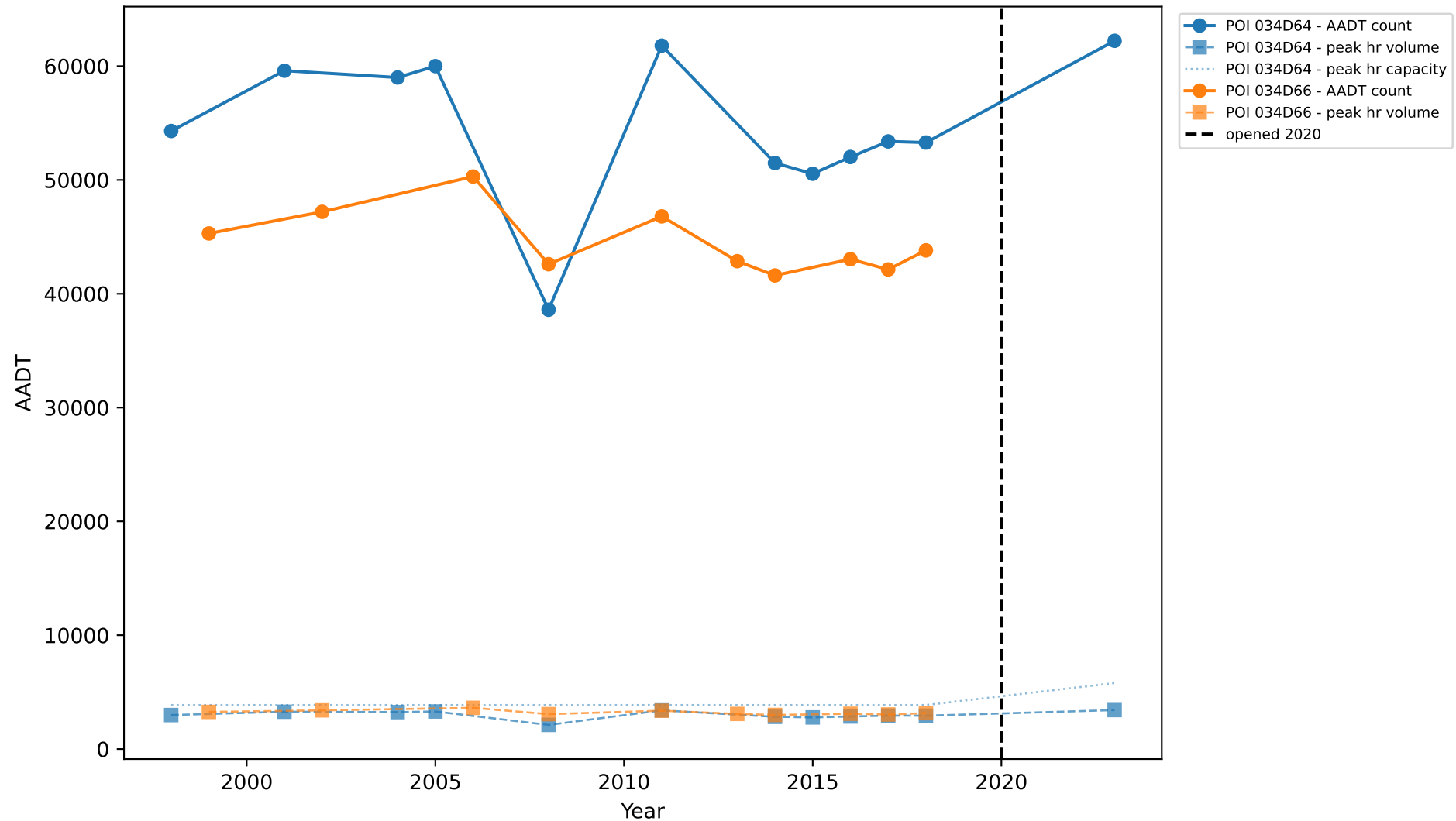
07-366.00: Traffic Counts, Peak Volume & Capacity by Station
