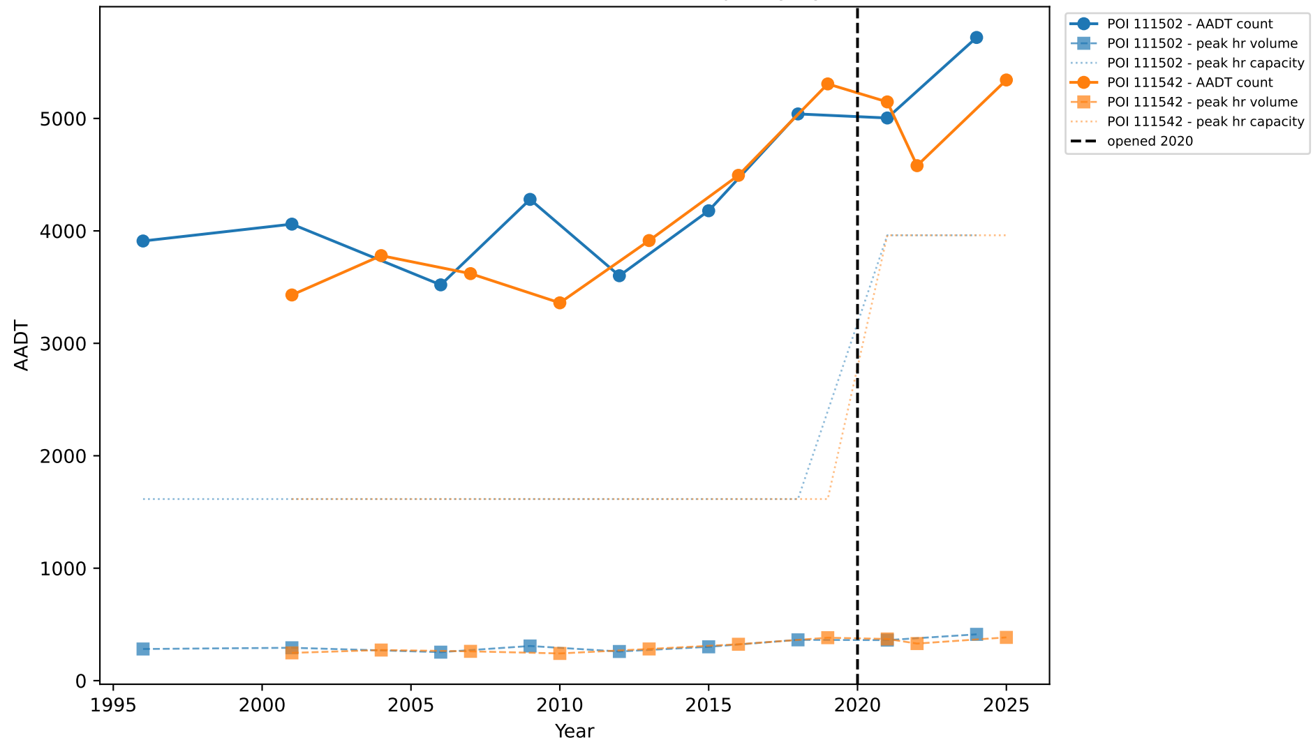
1-180.10: Traffic Counts, Peak Volume & Capacity by Station
