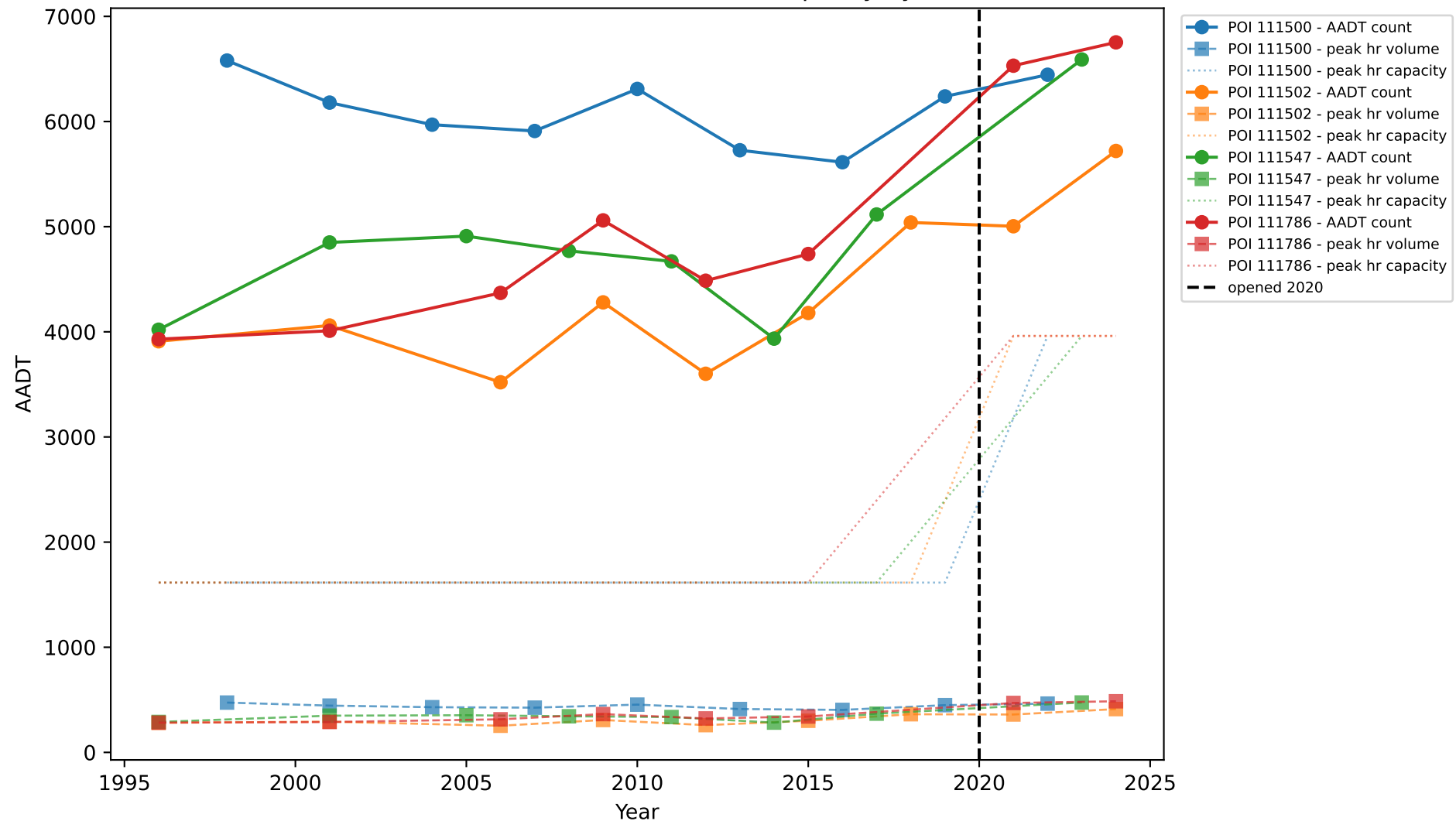
1-180.11: Traffic Counts, Peak Volume & Capacity by Station
