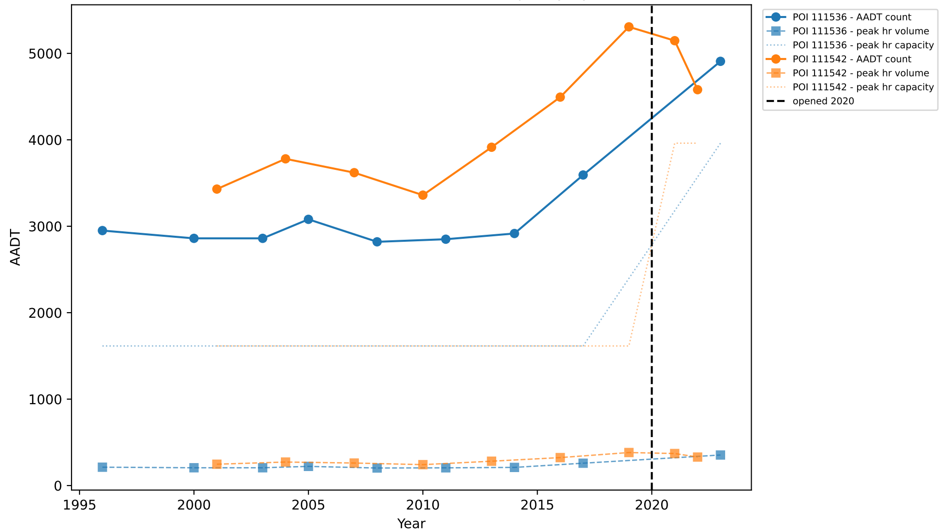
1-180.51: Traffic Counts, Peak Volume & Capacity by Station
