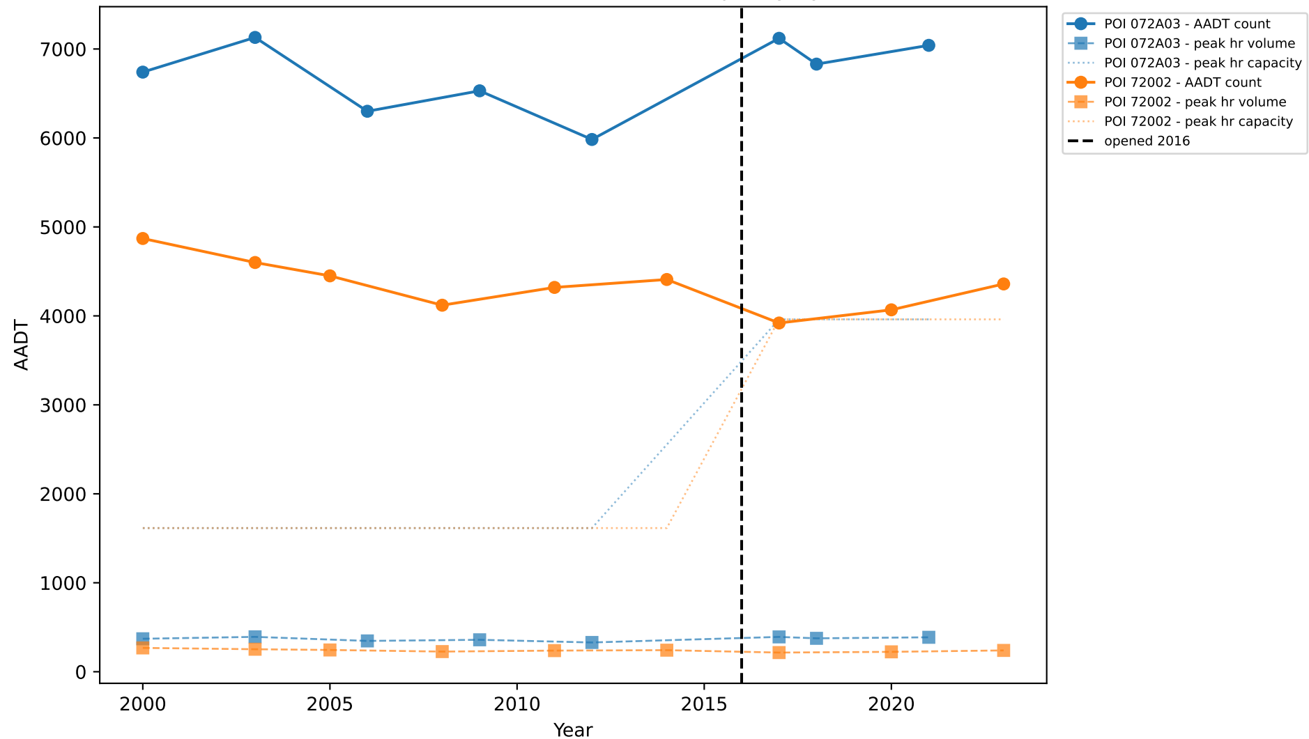
1-307.01: Traffic Counts, Peak Volume & Capacity by Station
