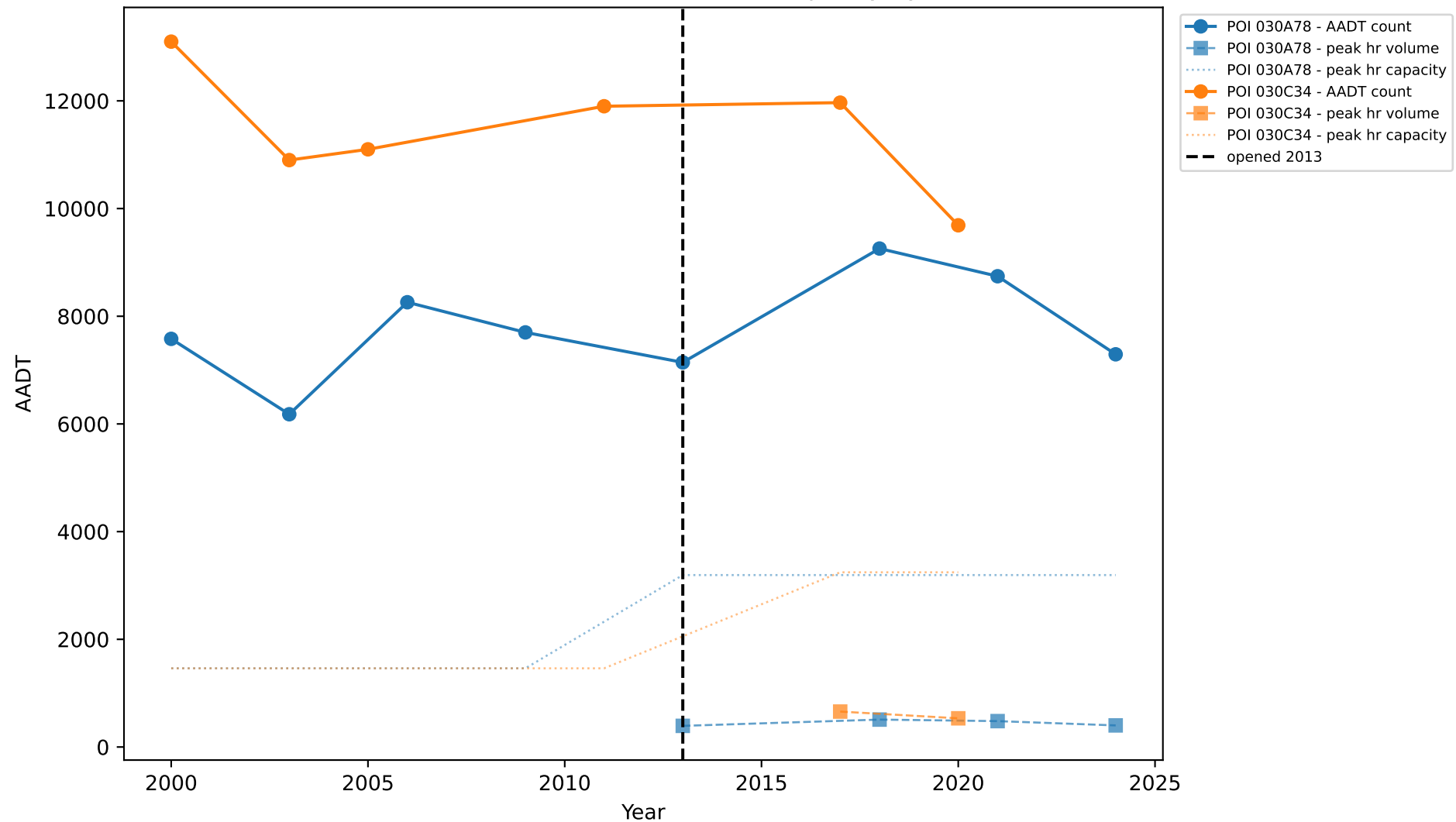
2-221.00: Traffic Counts, Peak Volume & Capacity by Station
