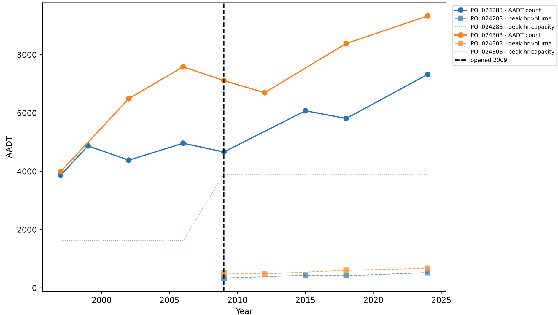
2-7000.00: Traffic Counts, Peak Volume & Capacity by Station
