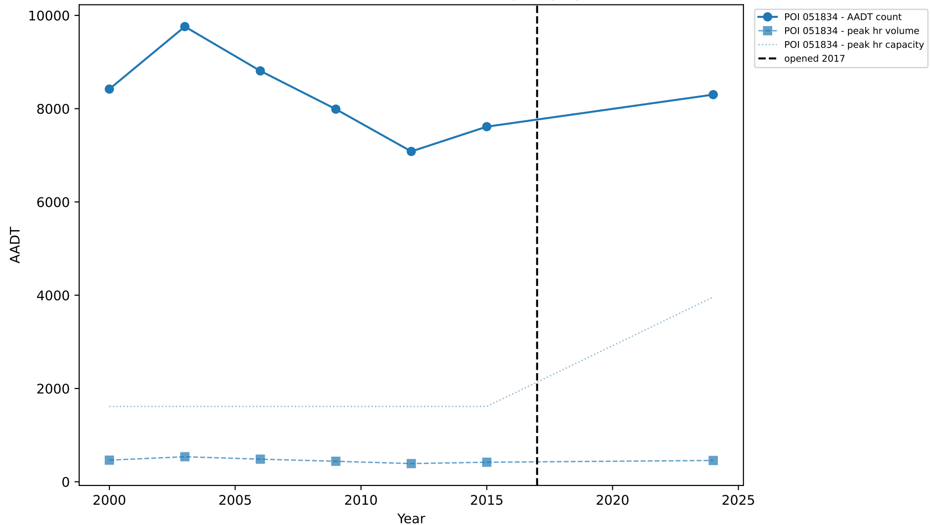
2-79.30: Traffic Counts, Peak Volume & Capacity by Station
