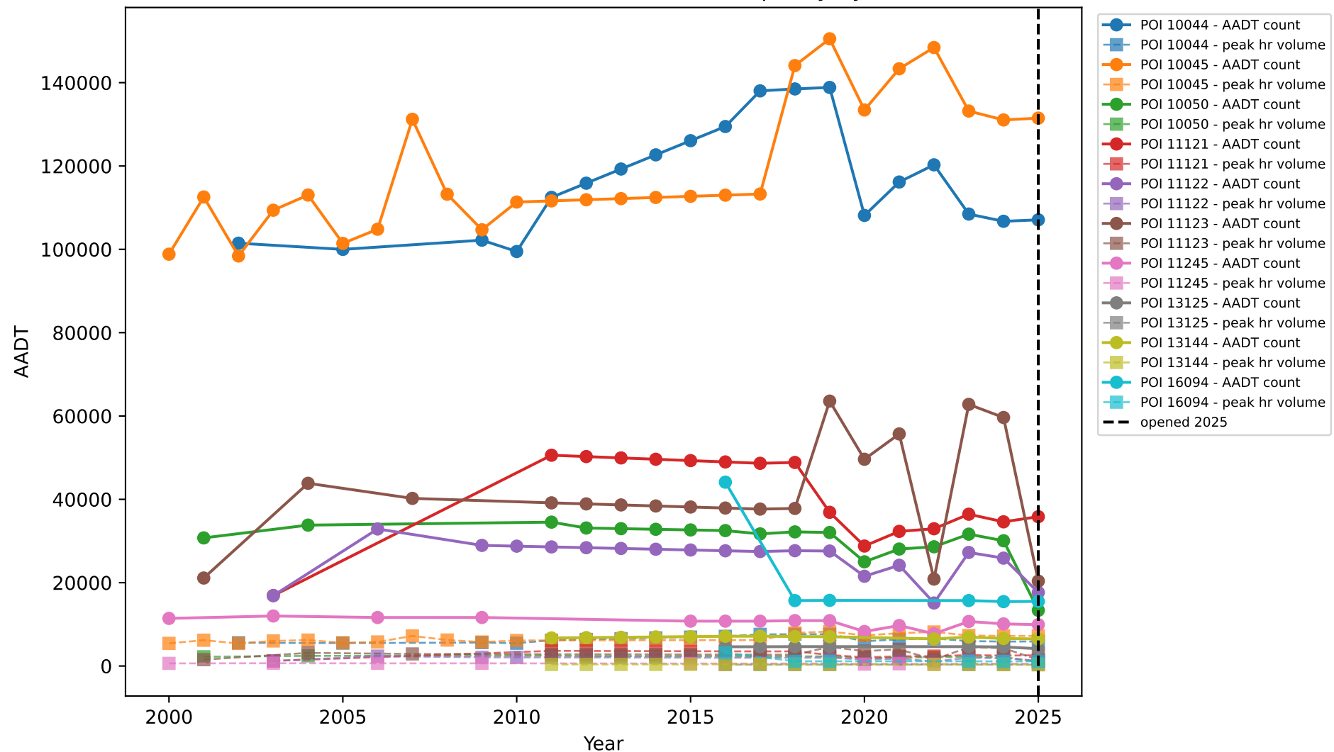
20190058: Traffic Counts, Peak Volume & Capacity by Station
