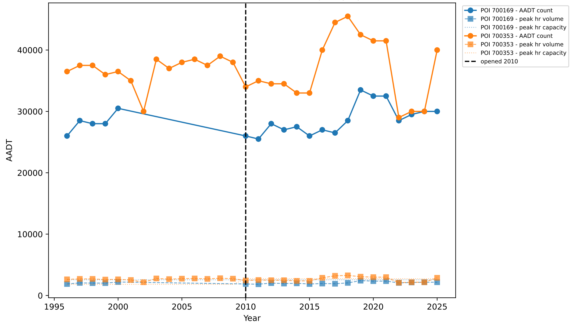
237576-1: Traffic Counts, Peak Volume & Capacity by Station
