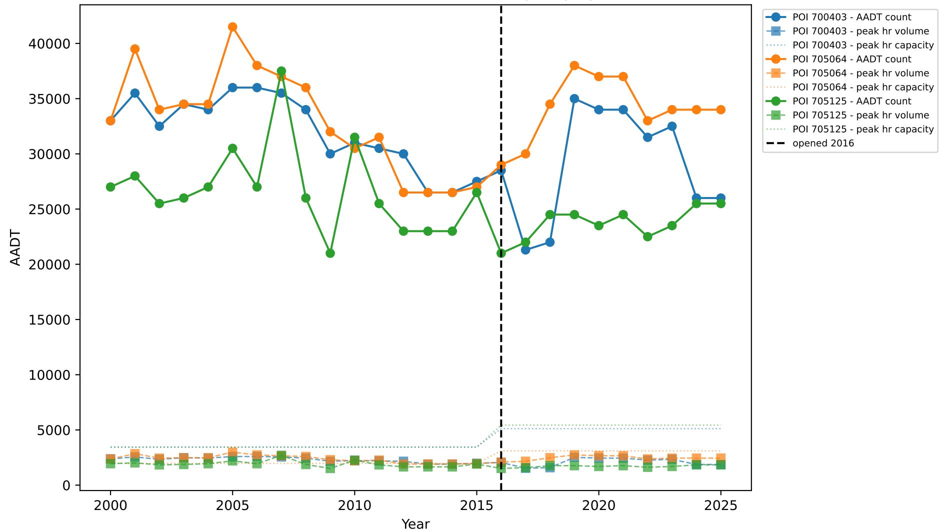
237592-1: Traffic Counts, Peak Volume & Capacity by Station
