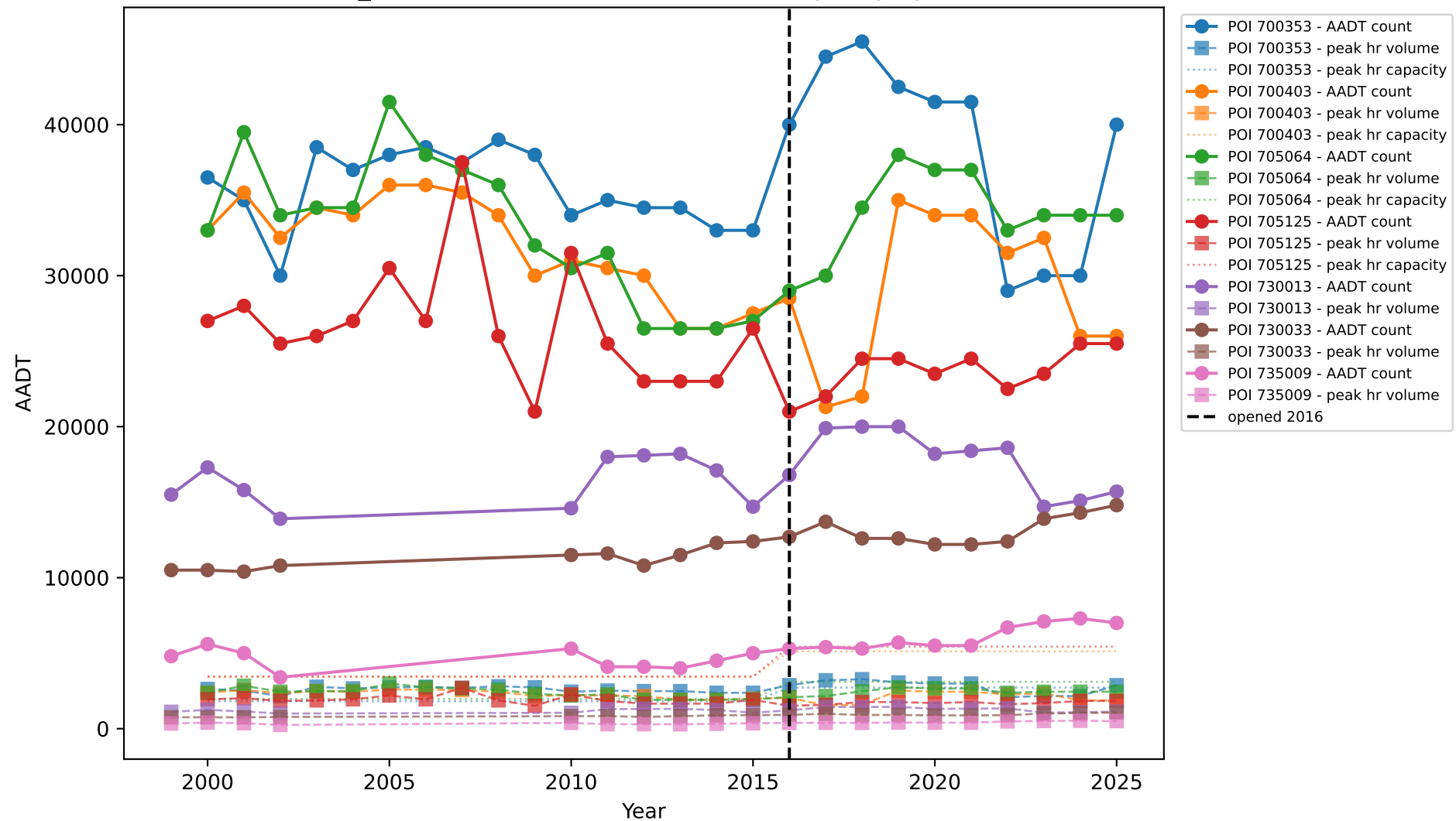
237592_2: Traffic Counts, Peak Volume & Capacity by Station
