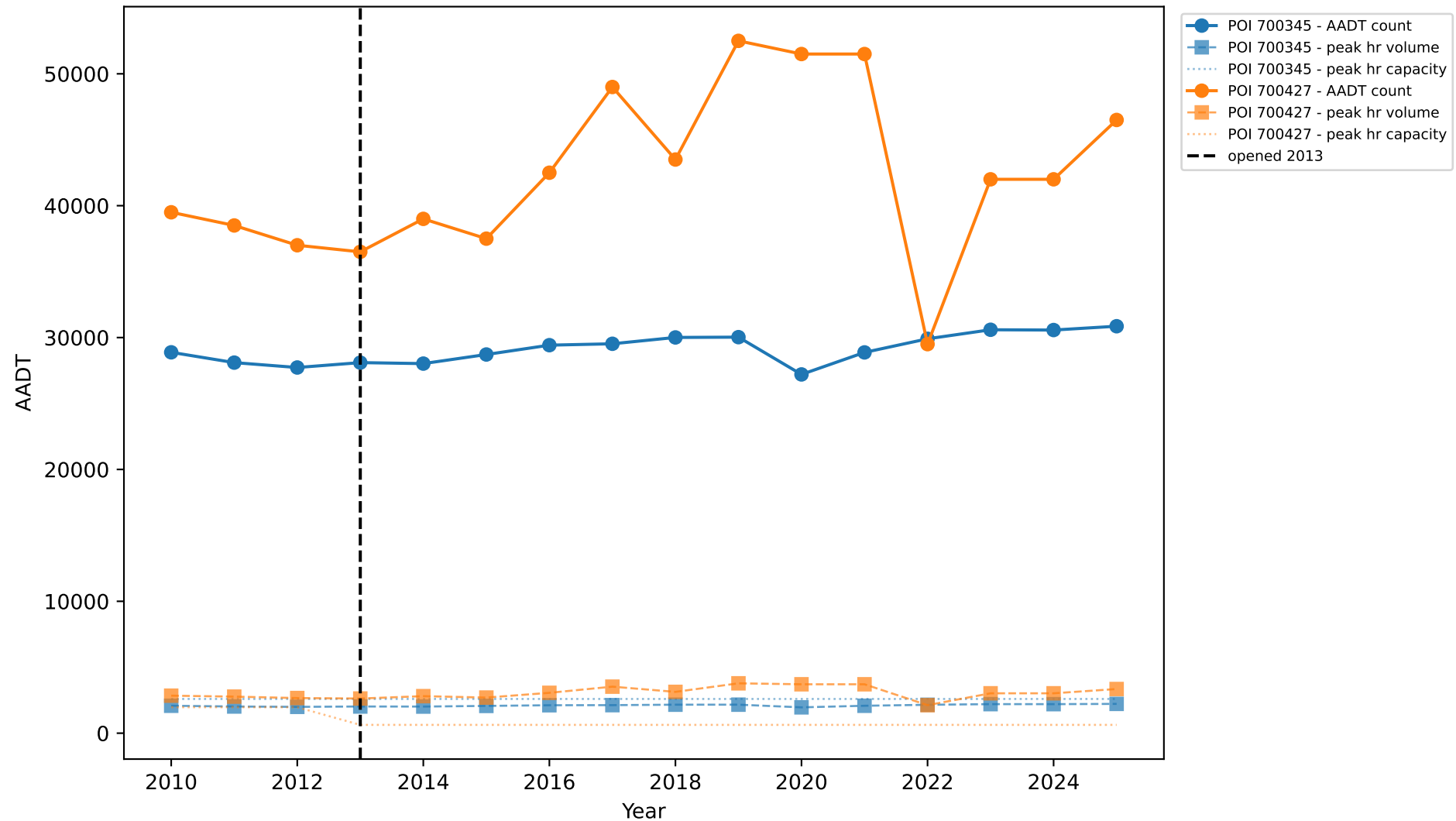
237650-3: Traffic Counts, Peak Volume & Capacity by Station
