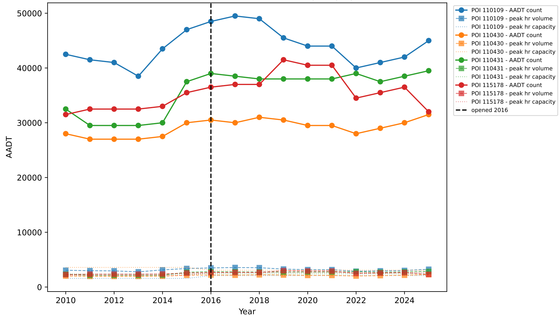
238395-4: Traffic Counts, Peak Volume & Capacity by Station
