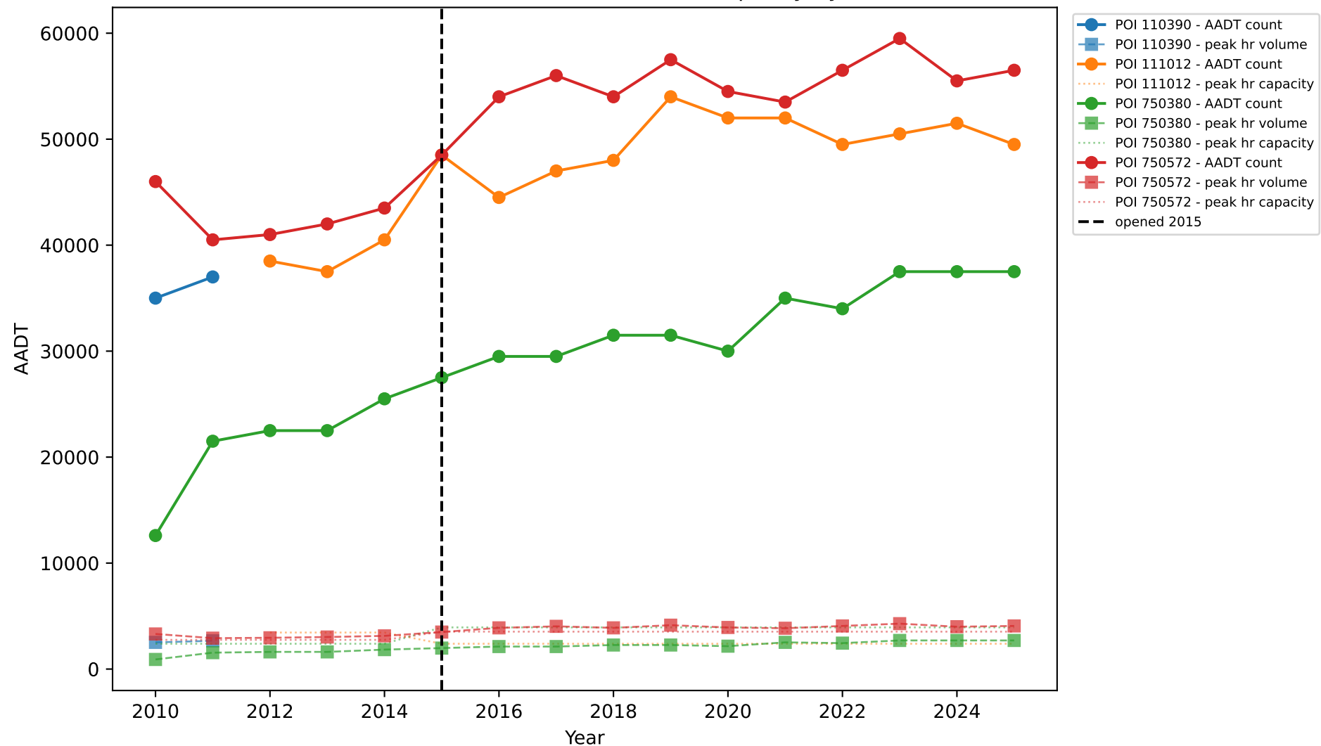
238429-4: Traffic Counts, Peak Volume &amp; Capacity by Station
