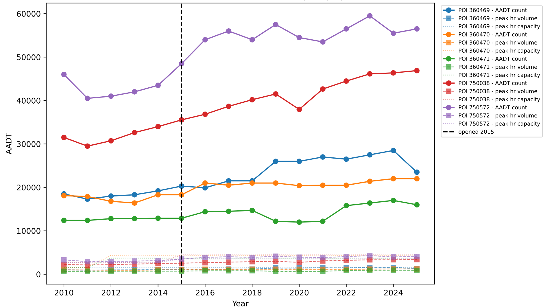
238429-5: Traffic Counts, Peak Volume & Capacity by Station
