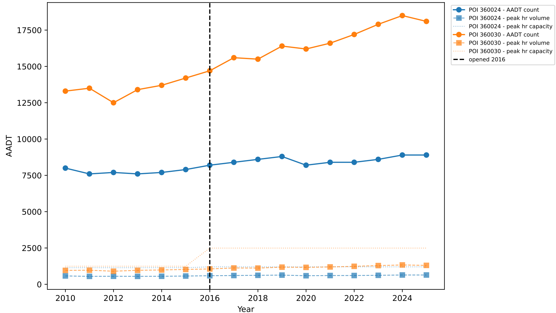
238720-1: Traffic Counts, Peak Volume & Capacity by Station
