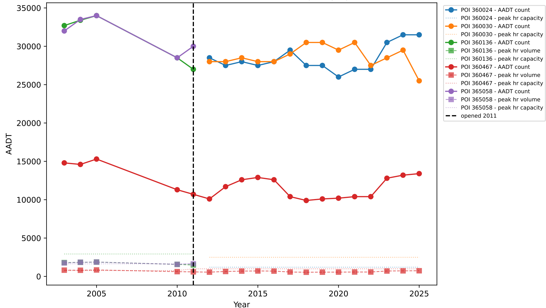
238753-1A: Traffic Counts, Peak Volume & Capacity by Station
