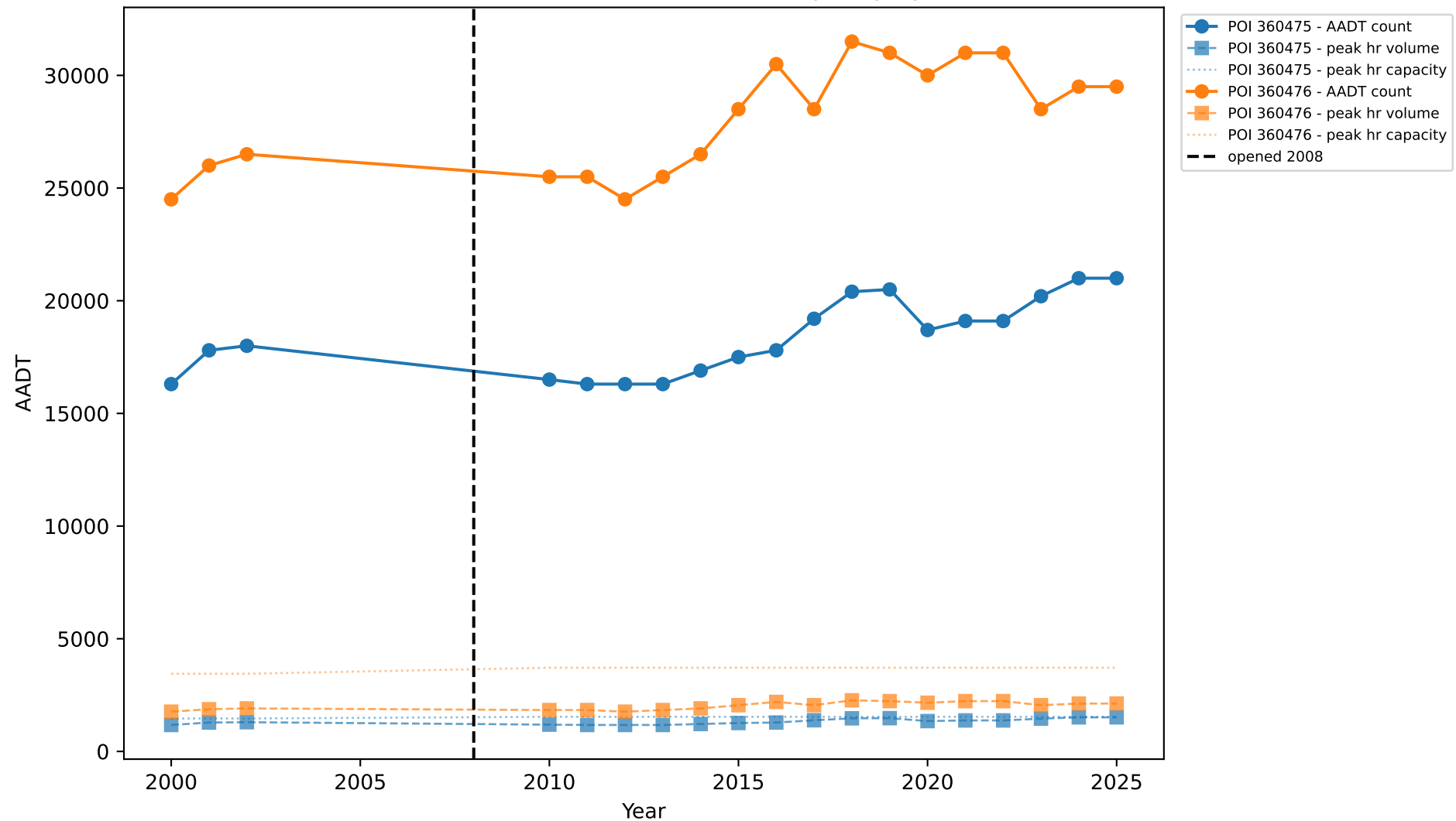
238762-1: Traffic Counts, Peak Volume & Capacity by Station
