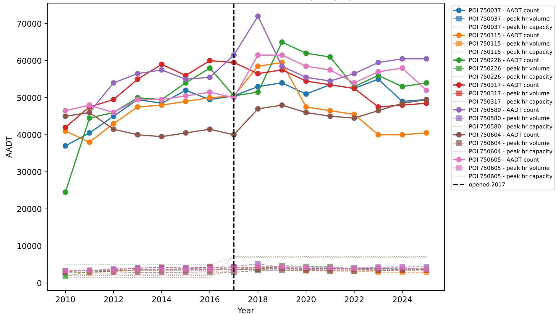
239203-2: Traffic Counts, Peak Volume & Capacity by Station
