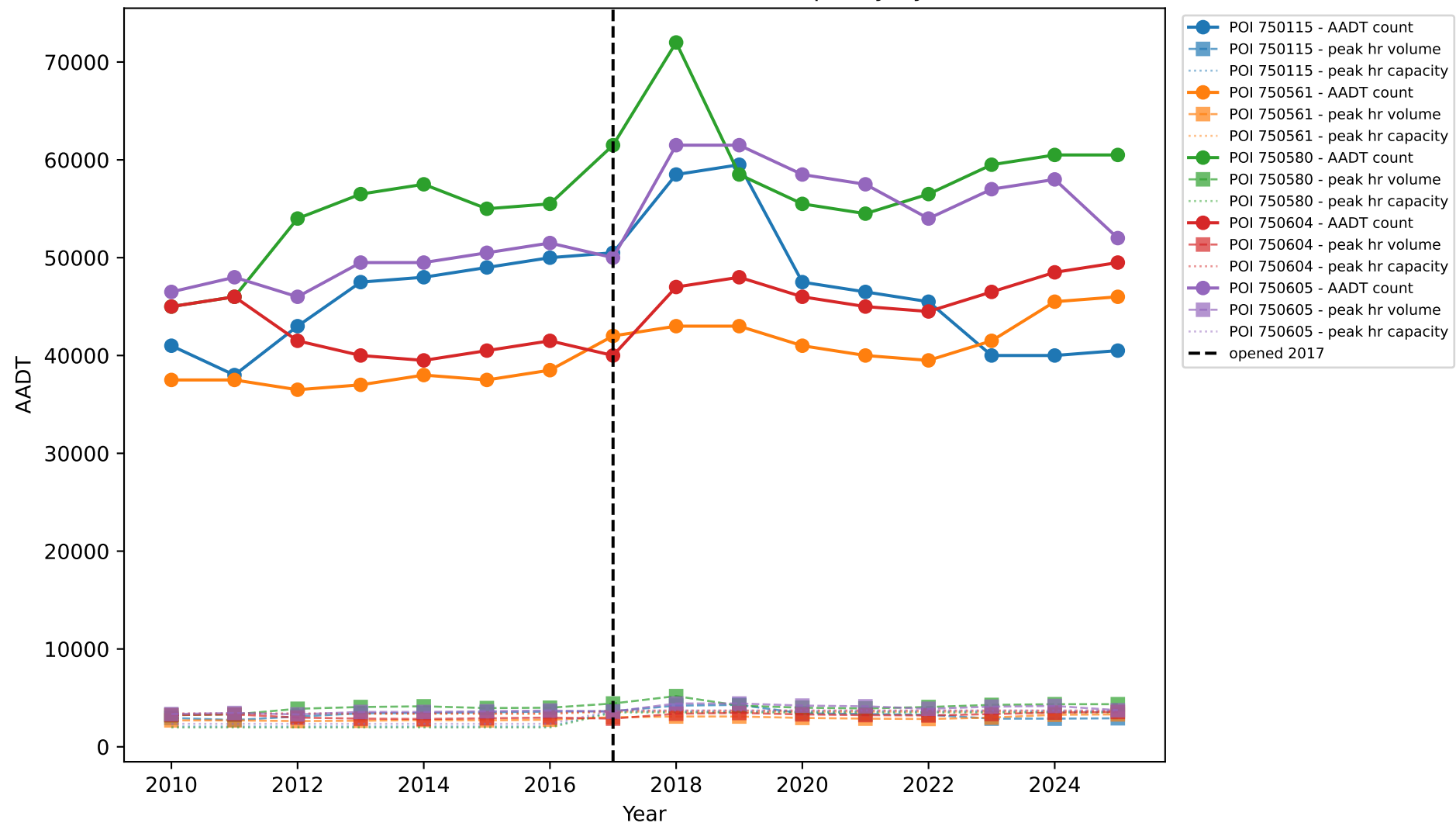
239203-4: Traffic Counts, Peak Volume & Capacity by Station
