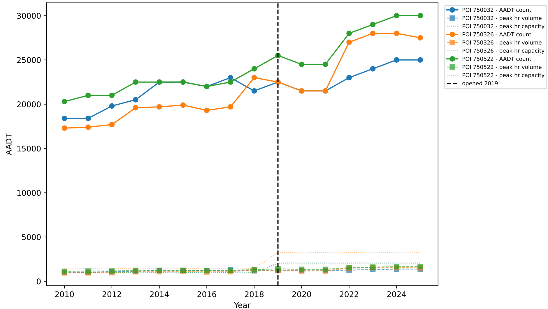
239266-3: Traffic Counts, Peak Volume & Capacity by Station
