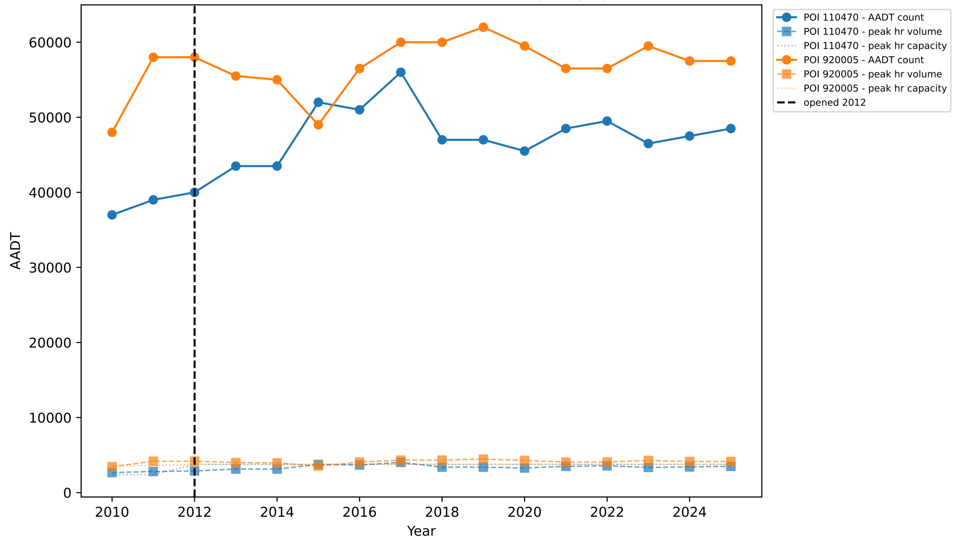
239304-1B: Traffic Counts, Peak Volume & Capacity by Station
