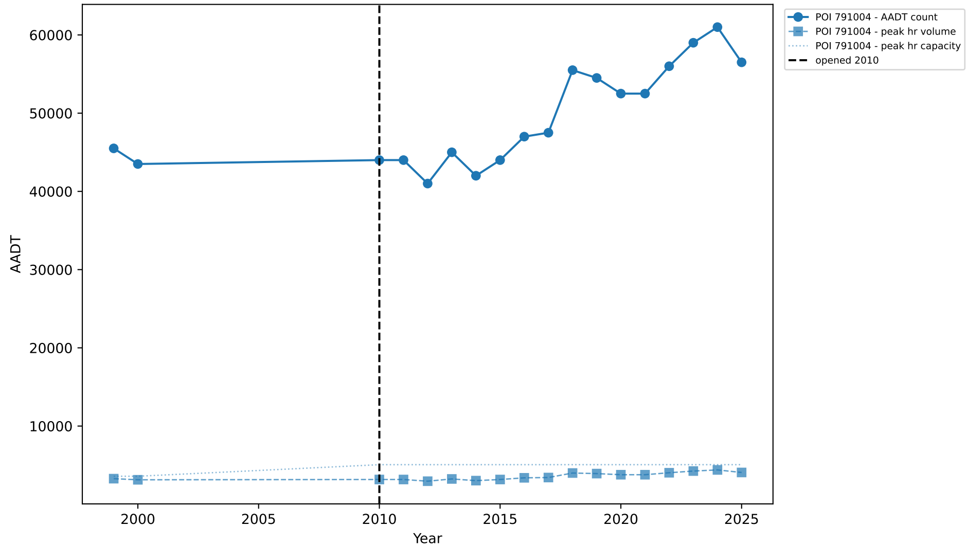
240887-1: Traffic Counts, Peak Volume & Capacity by Station
