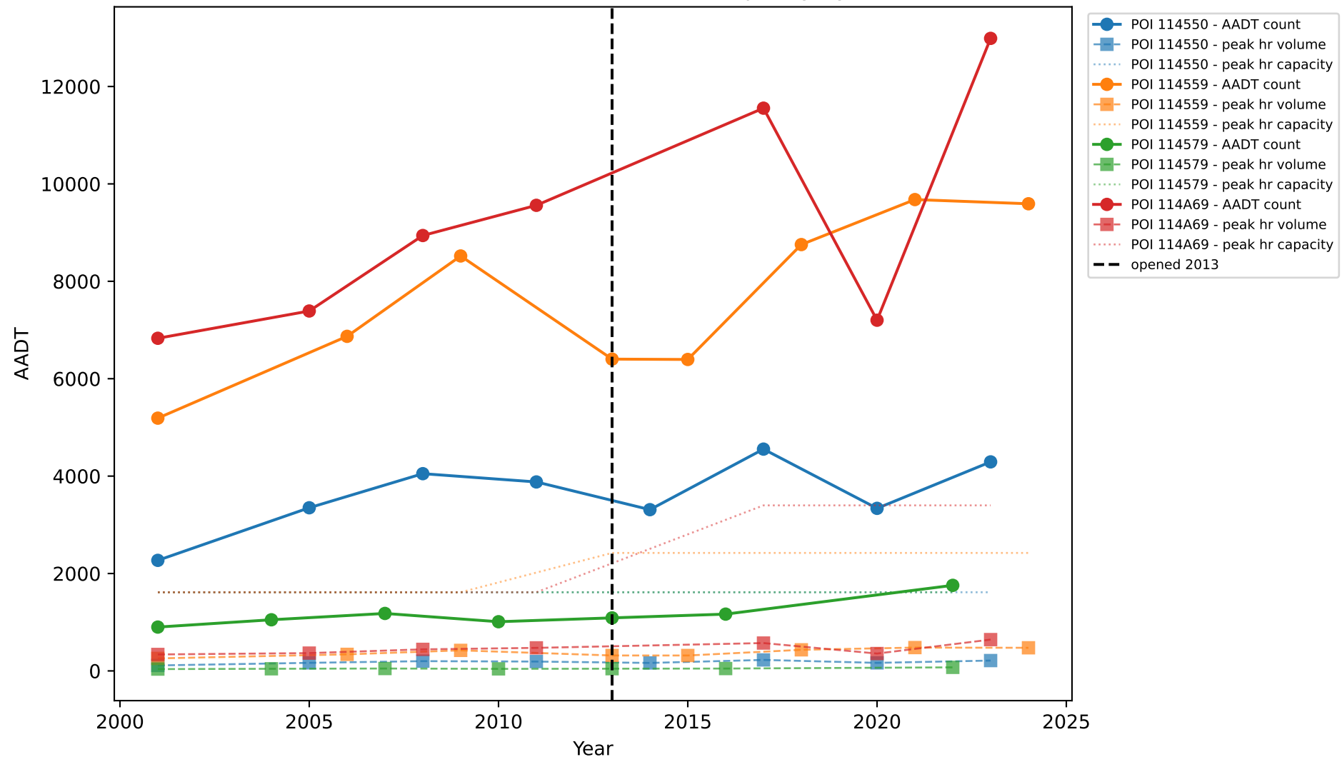
3-102.10: Traffic Counts, Peak Volume & Capacity by Station
