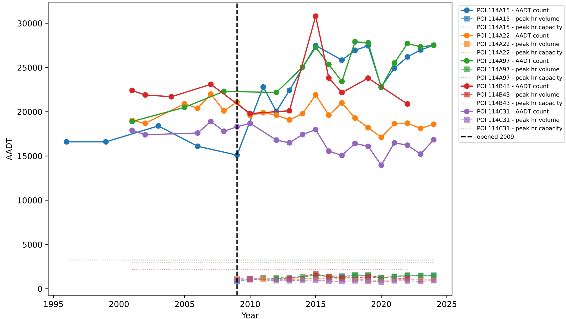
3-312.00: Traffic Counts, Peak Volume & Capacity by Station
