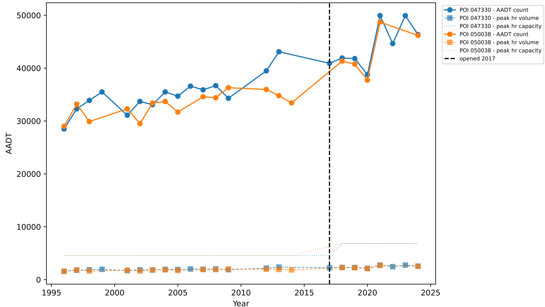
4-16.00: Traffic Counts, Peak Volume & Capacity by Station
