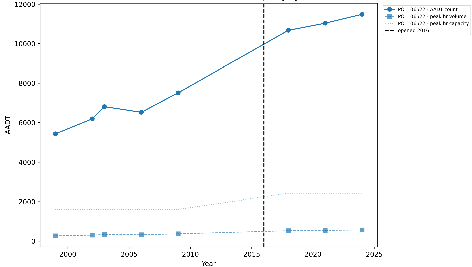
5-348.01: Traffic Counts, Peak Volume & Capacity by Station
