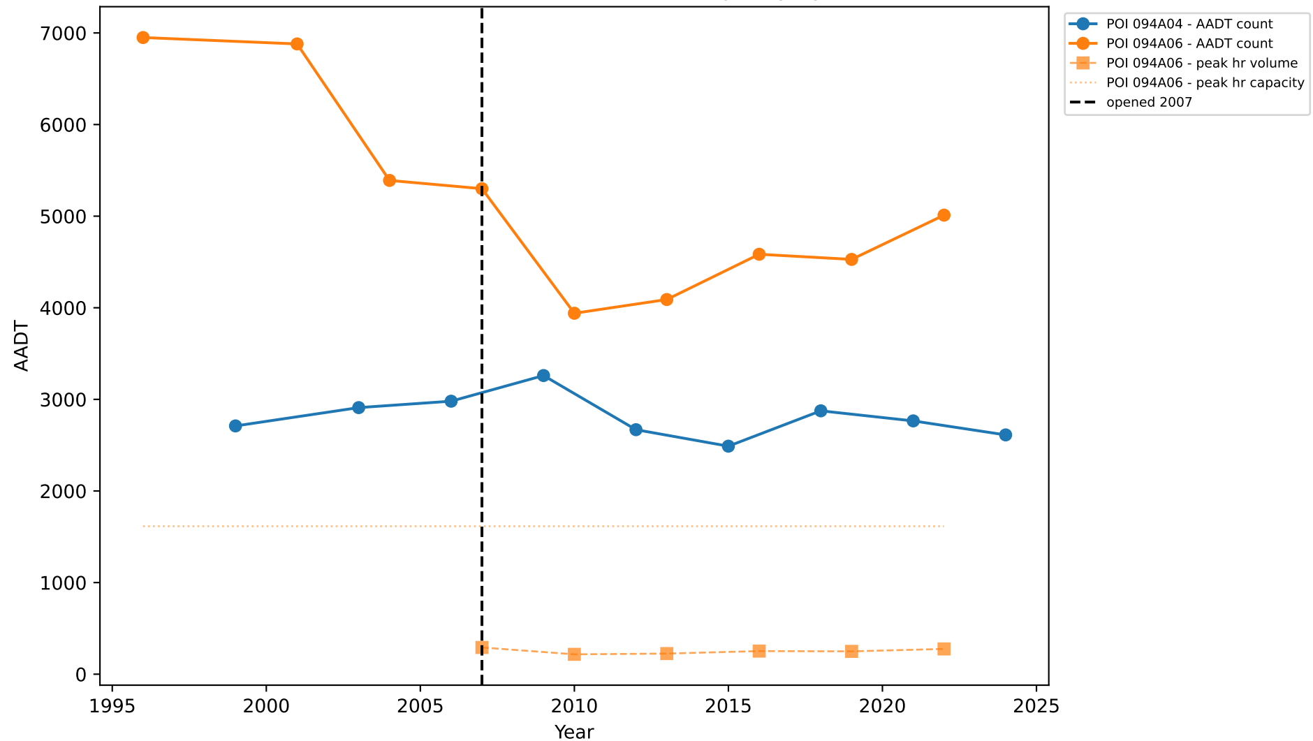
6-356.00: Traffic Counts, Peak Volume & Capacity by Station
