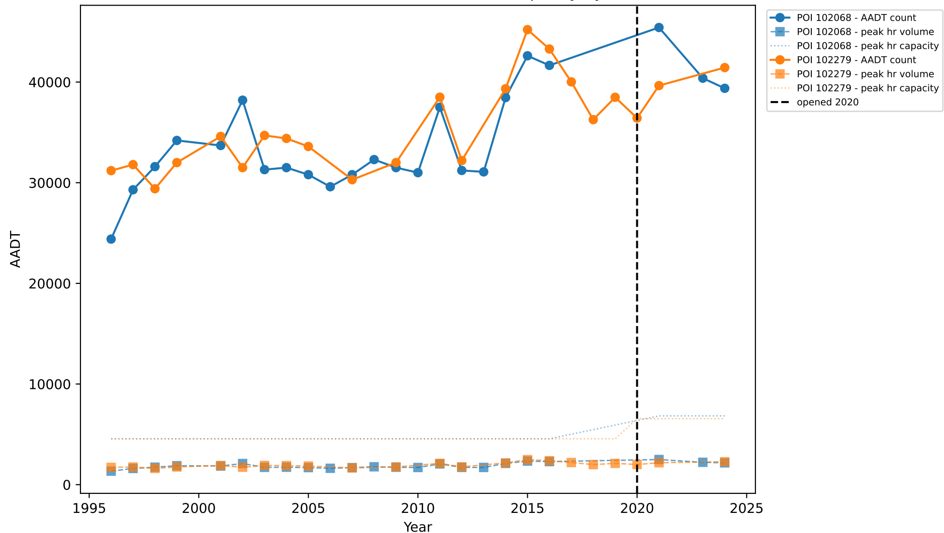
8-0006.10: Traffic Counts, Peak Volume &amp; Capacity by Station
