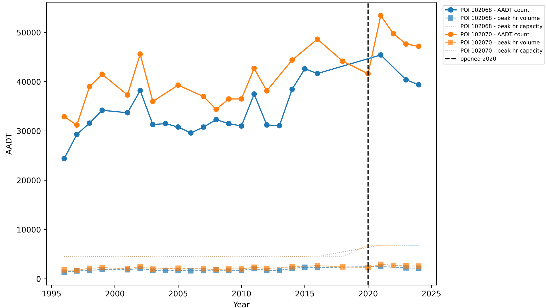
8-0006.20: Traffic Counts, Peak Volume & Capacity by Station
