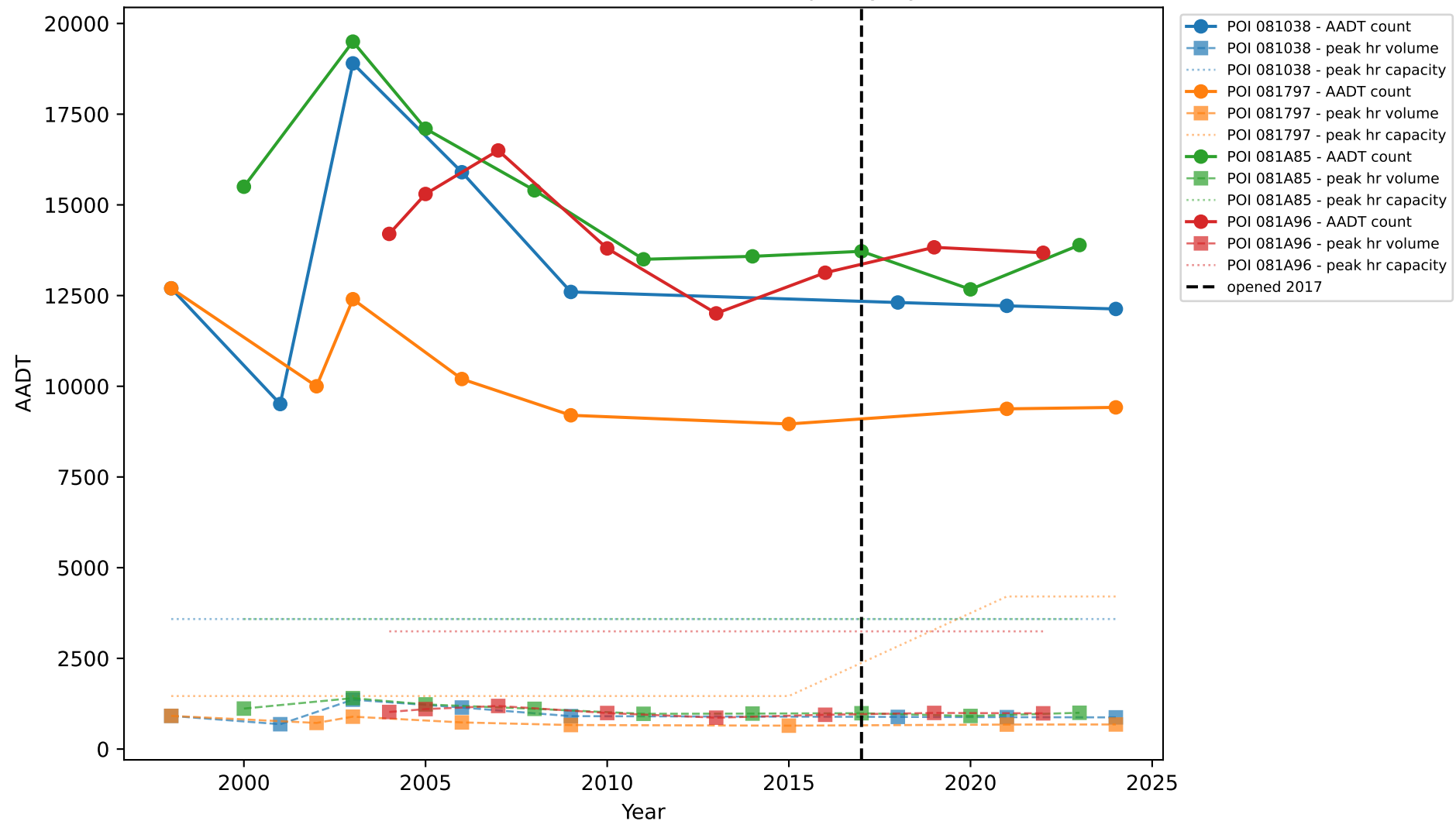
9-169.00: Traffic Counts, Peak Volume & Capacity by Station
